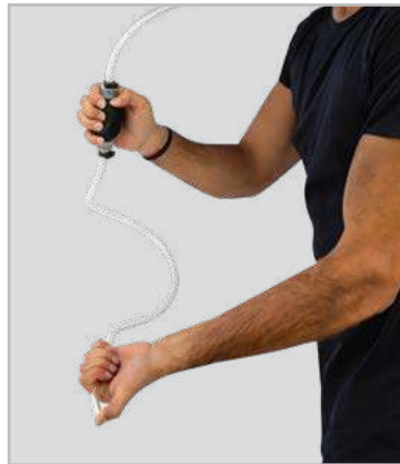
STEP - 3 Place your thumb over the bottom end of the discharge hose and squeeze the rubber pump a few times to start fluid transfer. Gravity does the rest
